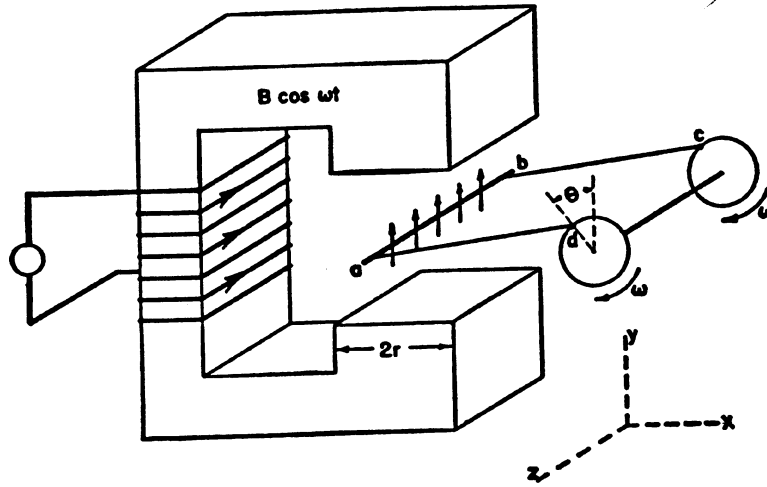
. Oscillating Bar Generator.
