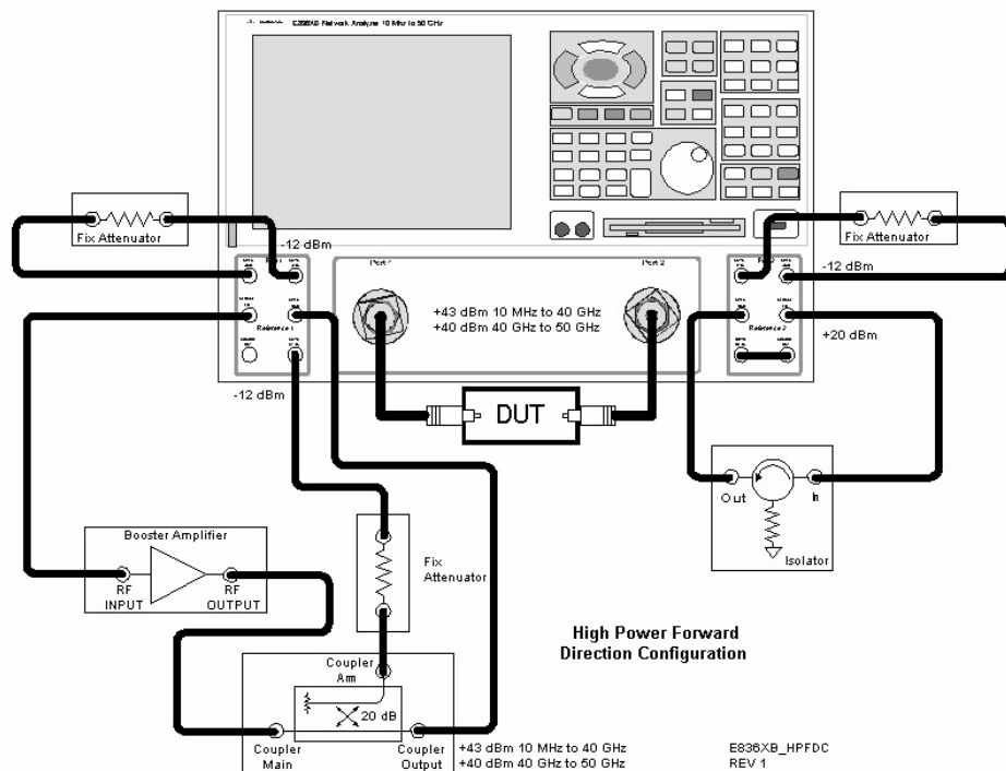
Figure 3 High Power One-way Input/Output
