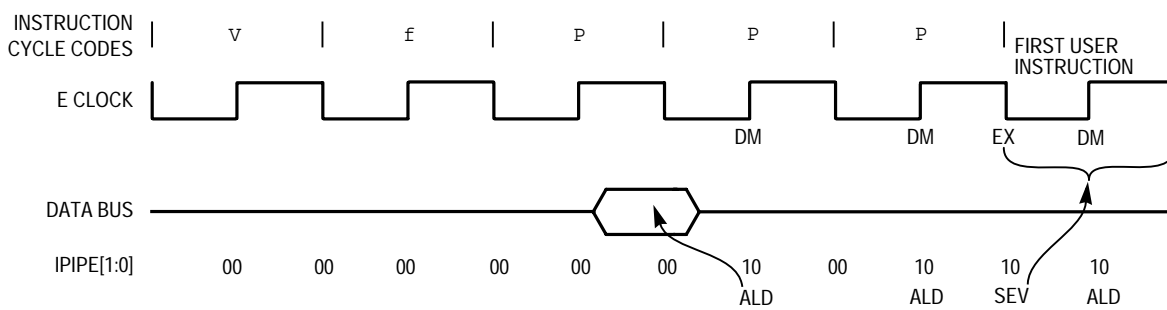
Figure 8-8. Reset Sequence for M68HC12
