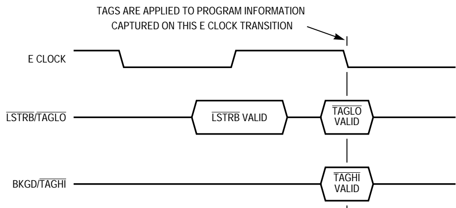
Figure 8-9. Tag Input Timing
