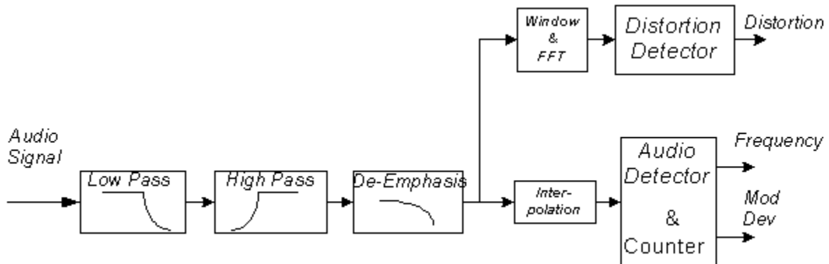
Figure 5-12 Audio Diagram
