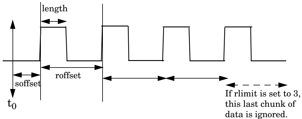
Figure 4-1 Sample Trace Data - Constant Envelope
