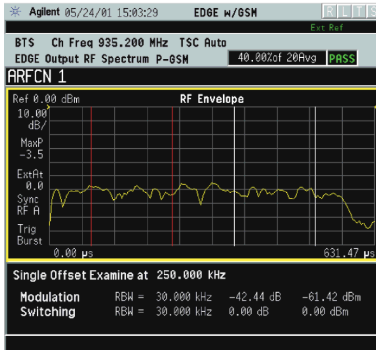
EDGE ORFS Result - Modulation with Single-Offset (Examine)
