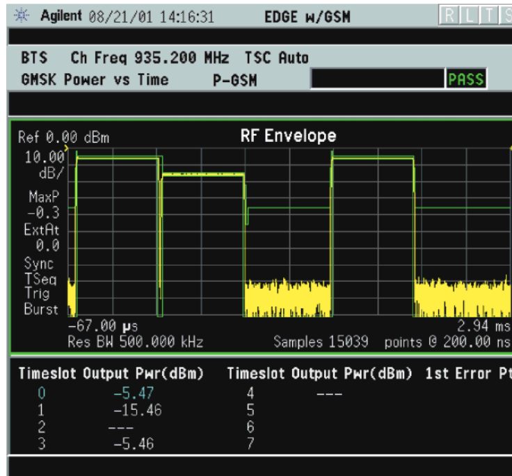
Figure 3-25 GSMK Power vs. Time Result - Multi-Slot View (5 slots shown)
