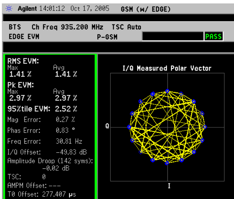
Figure 2-7 EDGE EVM Result - Polar Vector View
