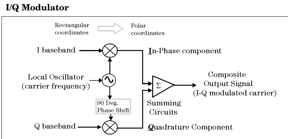
I-Q Modulator
