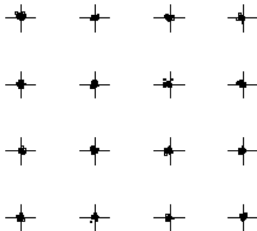
Figure 4-88 With Equalization
