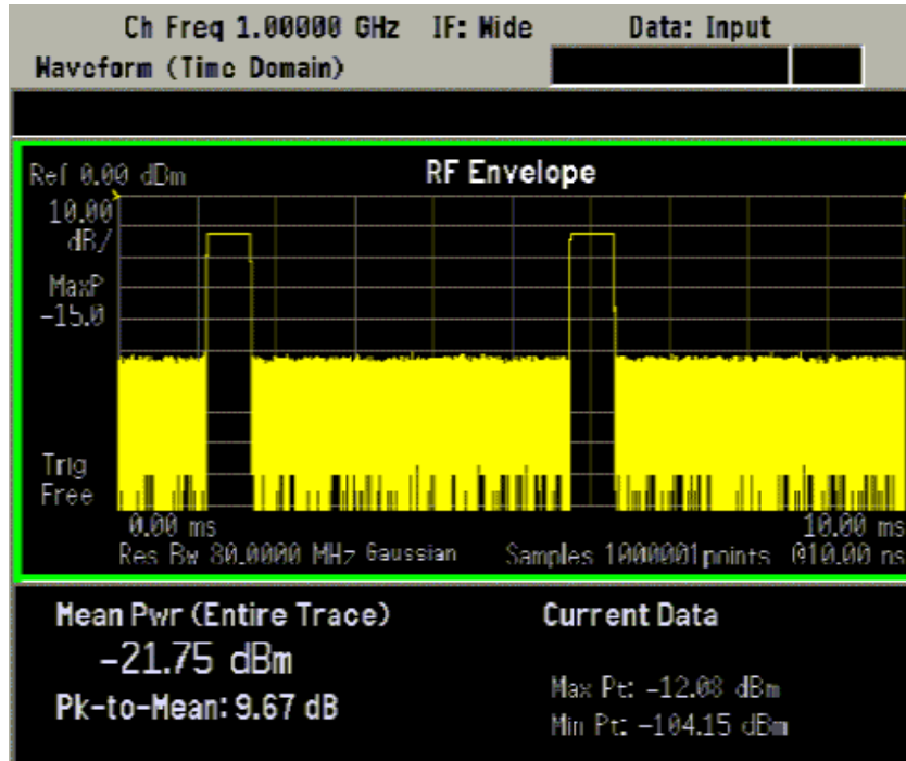
Figure 2-12 Waveform Measurement - RF Envelope View with Opt. 122– 80 MHz Bandwidth Digitizer Hardware
