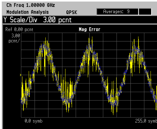
Figure 2-72 Magnitude Error Graph With PM Interference
