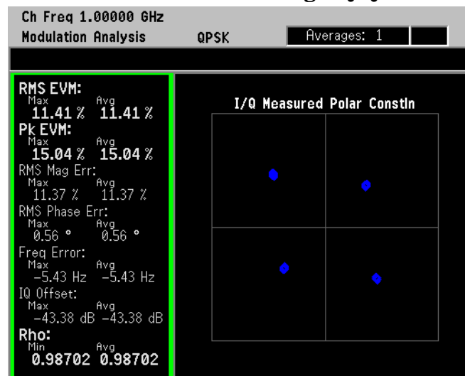
Figure 2-67 Polar Constellation Showing I/Q Quadrature Skew
