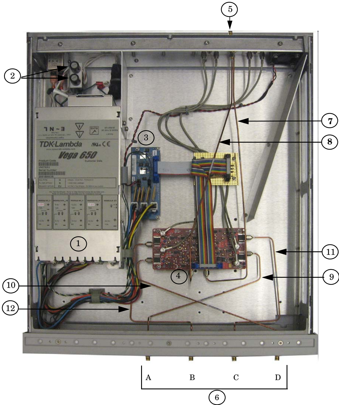
Figure 34 N5281A Option 700
