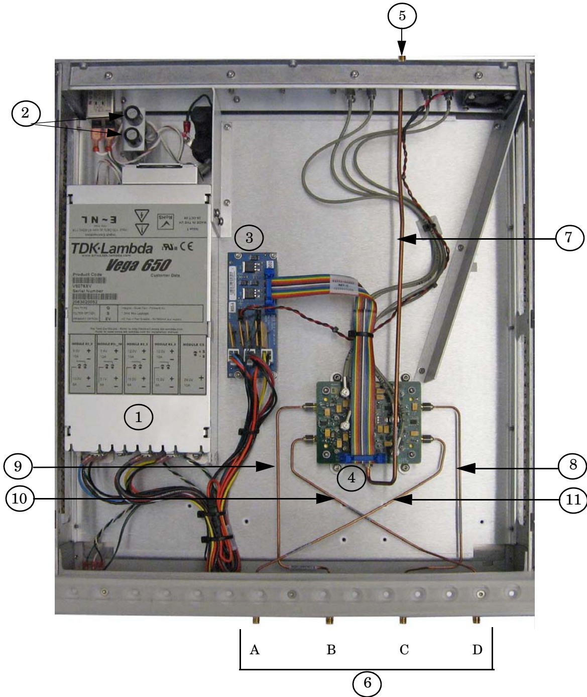
Figure 32 N5281A Option 700
