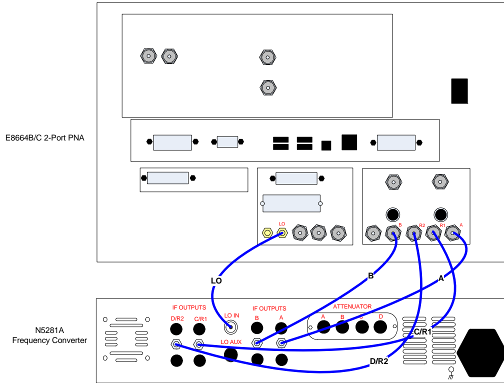
Figure 11 Rear Panel N5281A and E8364B/C
