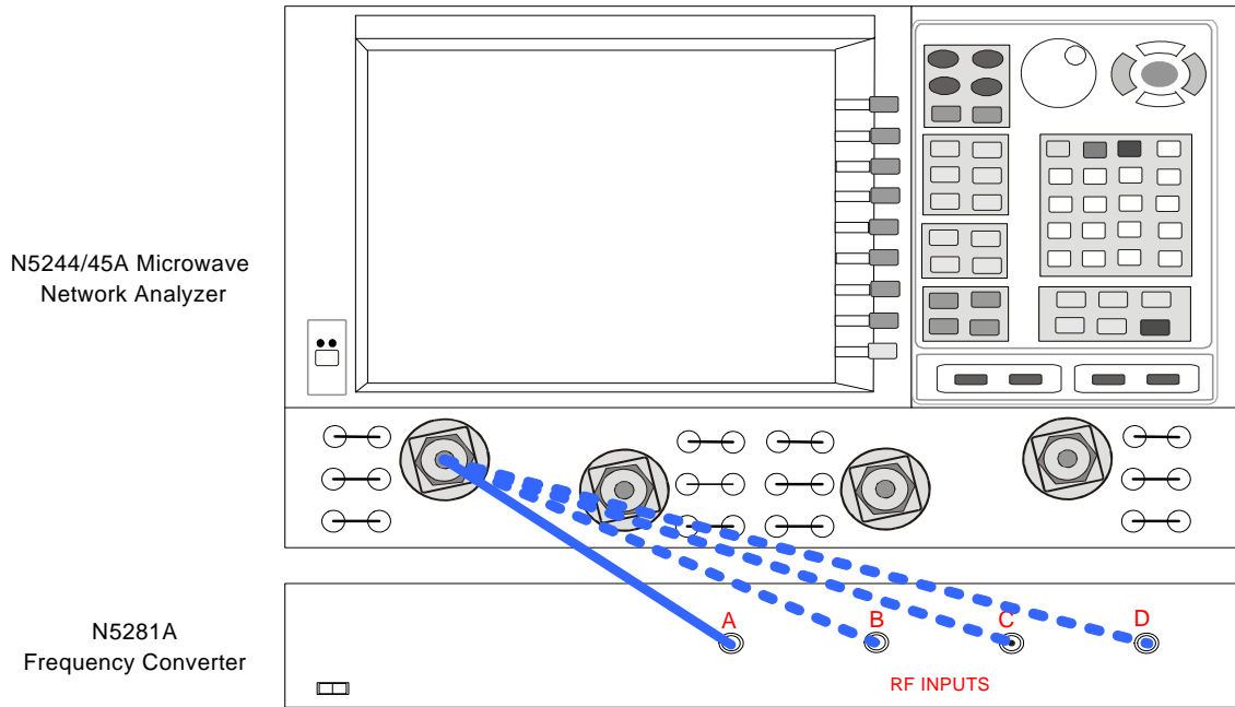
Figure 17 Front Panel N5281A and N5244/45A (4-Port)
